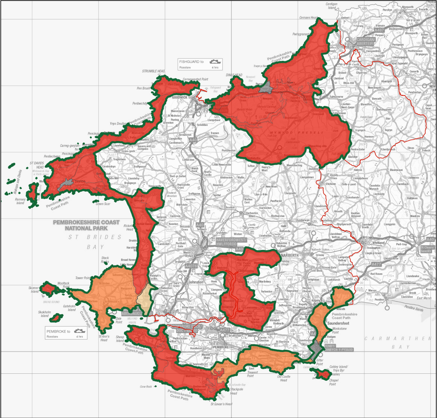
Figure 9.2: Landscape Sensitivity to Medium-scale Wind Turbines (25m - 65m to blade tip)
