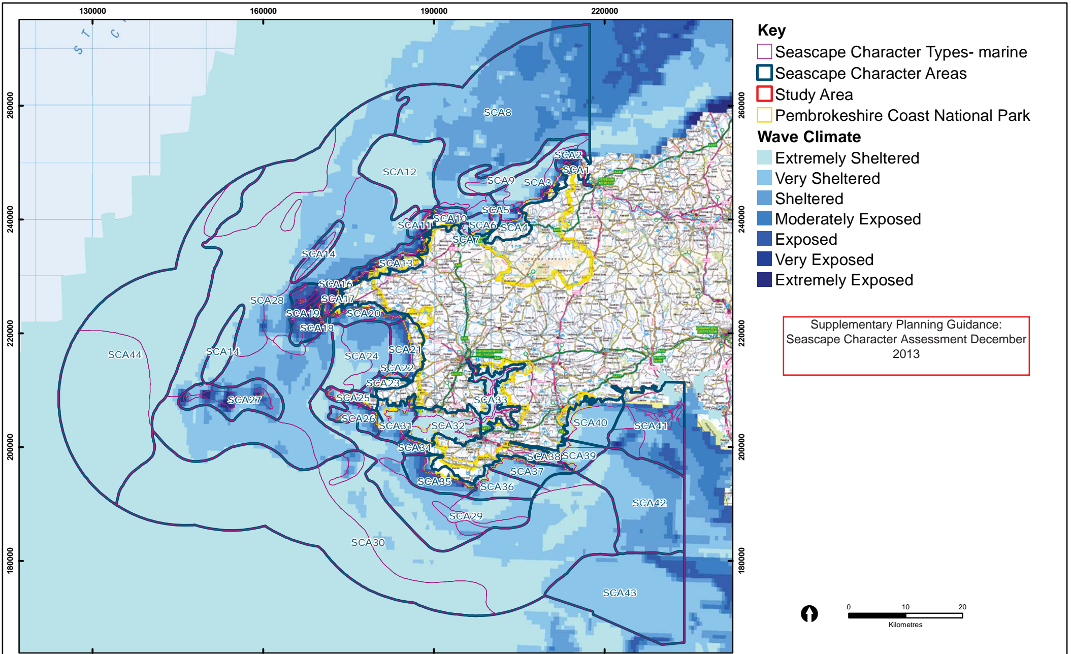
Figure 4: Wave Climate
