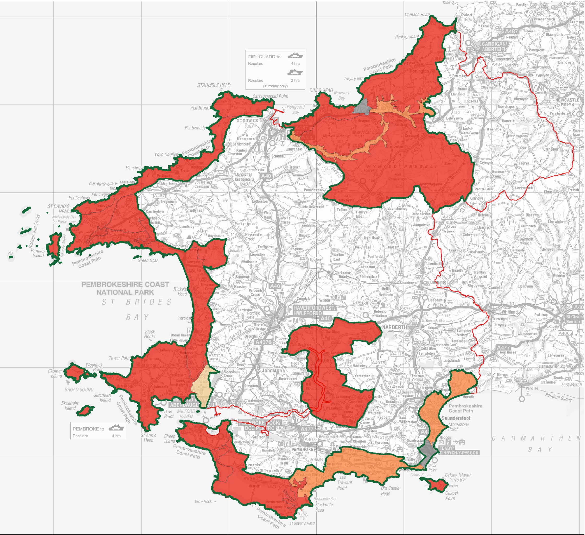
Figure 9.2: Landscape Sensitivity to Medium-scale Wind Turbines (25m - 65m to blade tip)
